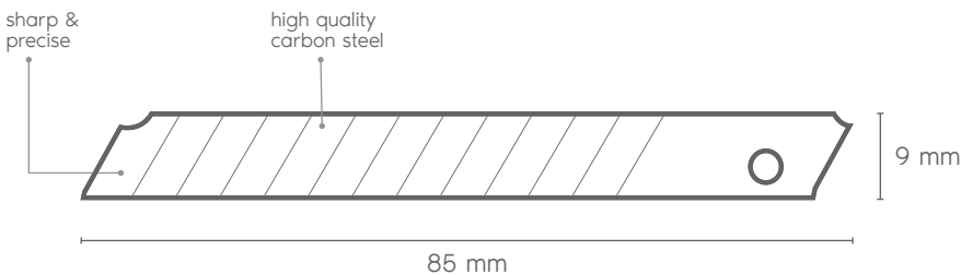
13 SERRATED SNAP SEGMENTS
